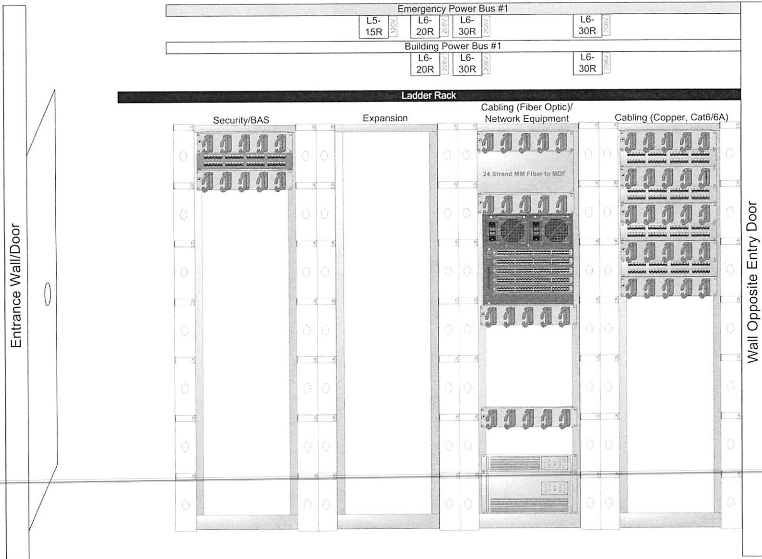
Figure 2: Sample IDF Rack Layout
